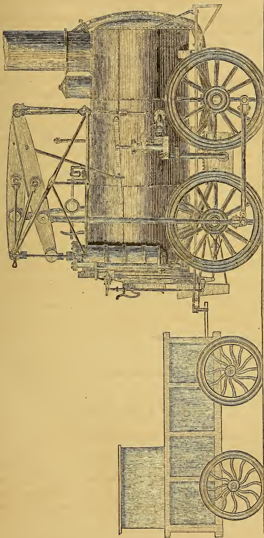
STOURBRIDGE LION.
