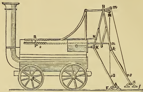
WILLIAM BRUNTON LOCOMOTIVE.
